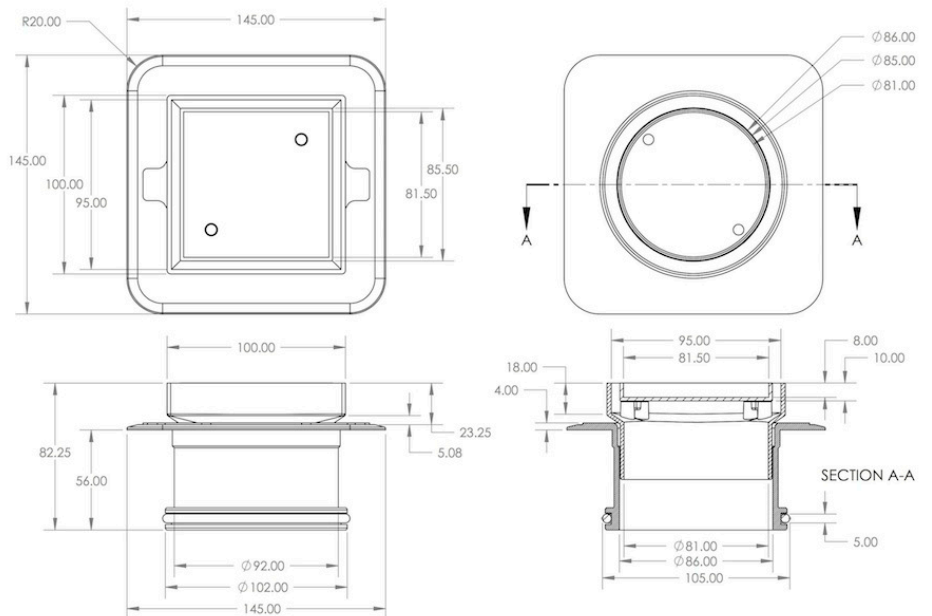
100mm SQUARE BERMUDA Mega Floor Grate
