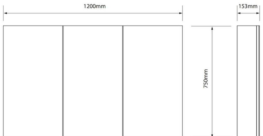
Mirror Cabinet -1200
